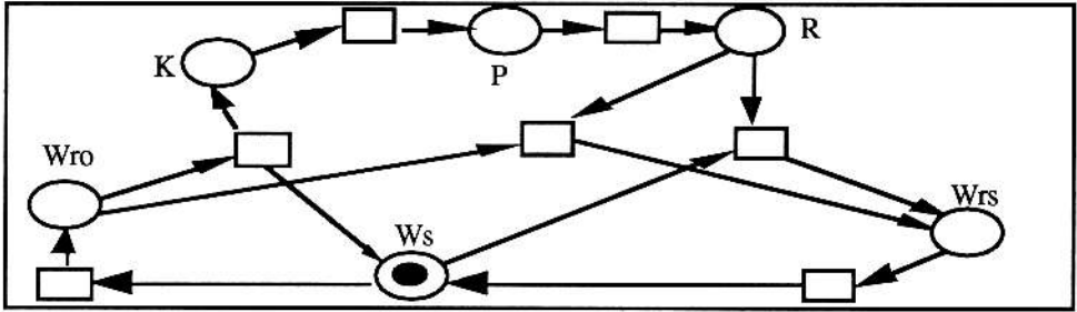
Figure 2: Specification and solution to the task "Bavarian biergarten"
