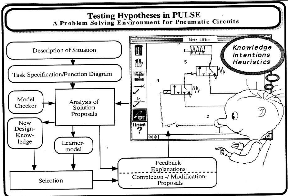
Figure 1: The Intelligent Design Environment PULSE
