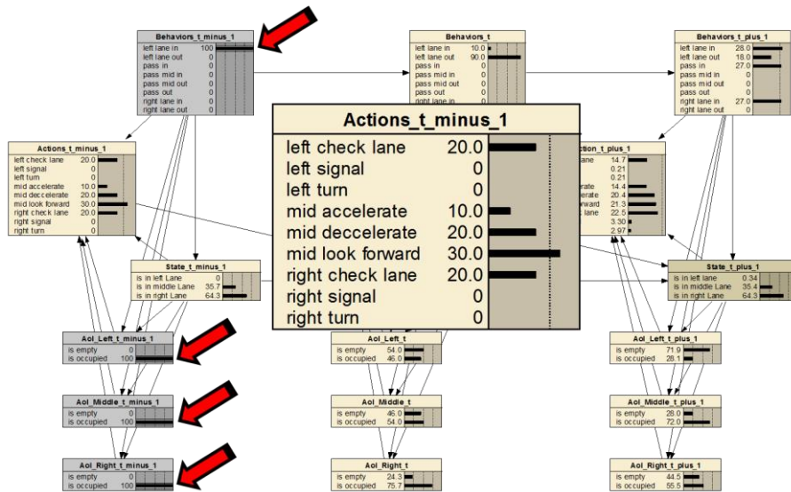
FIGURE 7 Conditional distributions in Dynamic Reactive MoB Model when receiving a combination of Behavior (goal) and blocking AoI evidence (Action-node expanded)
