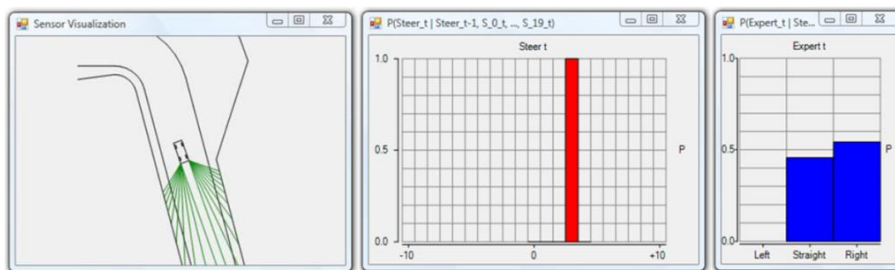
Fig. 10 Ambient perceptual evidence (left) and conditional distributions (middle, right) in Dynamic Partial Inverted BAD-MoB-model with 2 Bayesian Classifiers when leaving a right bended curve
