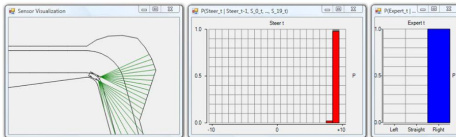
Fig. 9 Ambient perceptual evidence (left) and conditional distributions (middle, right) in Dynamic Partial Inverted BAD-MoB-model with 2 Bayesian Classifiers when driving in a right bended curve
