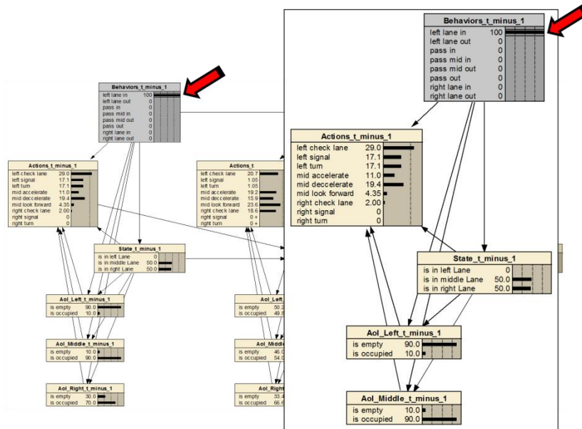
FIGURE 6 Expected behavior of the 3-TBN model with the goal behavior left_lane_in (the left-upper part of time-slice t-1 is expanded on the right of the figure)
