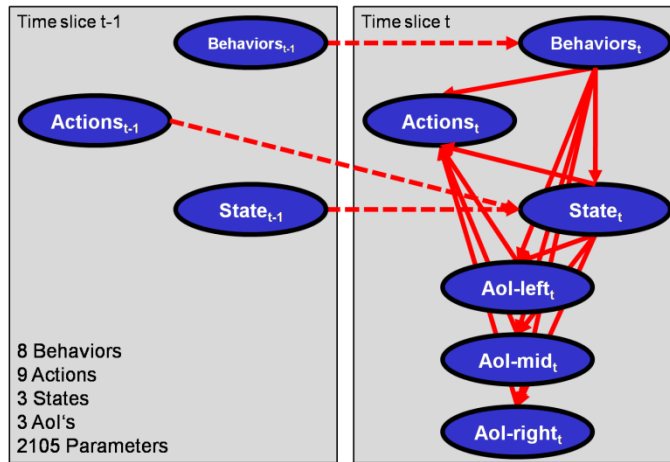
FIGURE 5 Dynamic Reactive BAD-MoB-model with Behavior and State Classifiers
