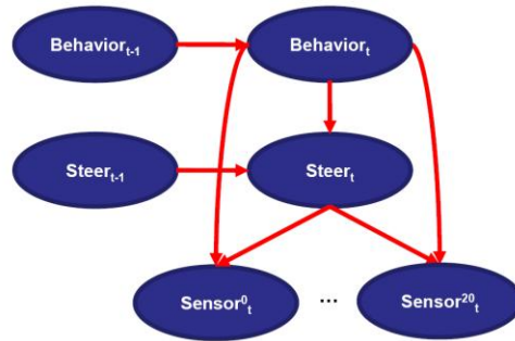
FIGURE 8 Dynamic BAD-MoB-model with Bayesian Classifiers Behavior and Steer
