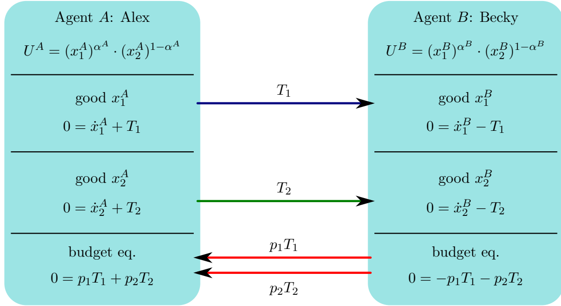
Figure 1: Structure of simple exchange model. Two agents A and B with utility functions U^A and U^B own stocks x_1^A, x_2^A, x_1^B , and x_2^B of good x_1 with price p_1 and x_2 with price p_2 . T_i corresponds to a transfer of good i from A to B .
