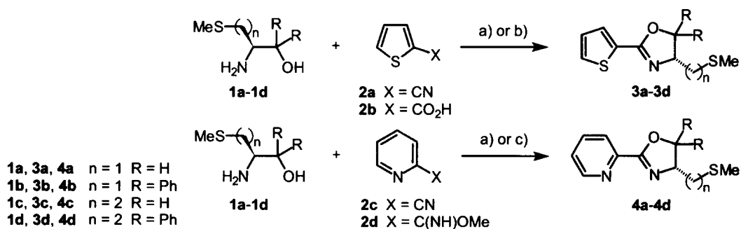
Scheme 1. Formation of oxazolines from 1.0 eq. amino alcohol 1 and 1.0 eq. carboxylic acid derivative 2 ; reagents and conditions: a) 0.03–0.05 eq. \text{ZnCl}_2 , \text{PhCl} , 16 h, 135^\circ\text{C} ; b) 3 eq. \text{PPh}_3 , 4 eq. \text{CCl}_4 , 4 eq. \text{NEt}_3 , pyridine– \text{MeCN} (1 : 1), 24 h, room temp.; c) cat. \text{HCl-H}_2\text{O} , \text{PhCl} , 24 h, 80^\circ\text{C} .
