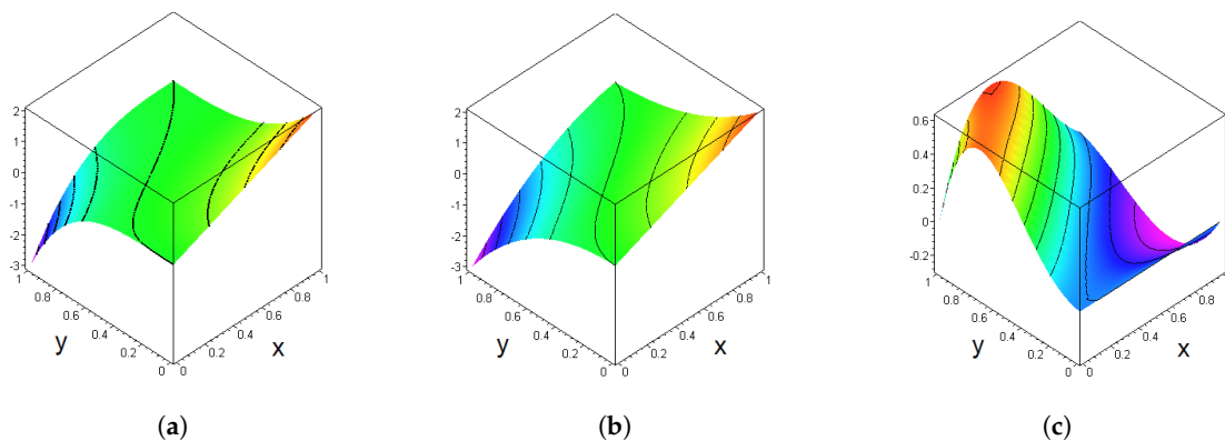
Figure 1. Plots of the functions in Example 1. (a) Plot of f(x, y) . (b) Plot of B_n f(x, y) . (c) Plot of f(x, y) - B_n f(x, y) .
