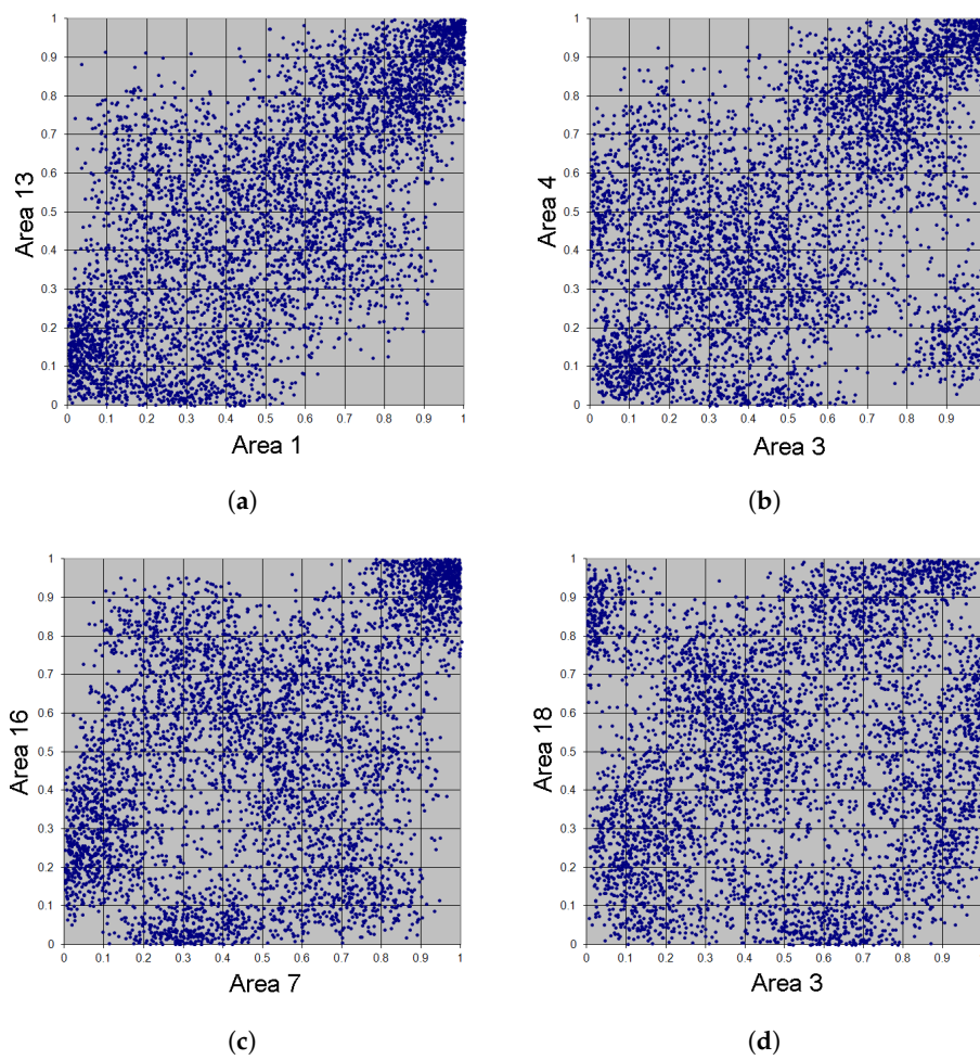
Figure 13. Simulation of 5000 adaptive Bernstein copula points in Example 5, m = 20 . (a) Area 1 vs. Area 13. (b) Area 3 vs. Area 4. (c) Area 7 vs. Area 16. (d) Area 3 vs. Area 18.
