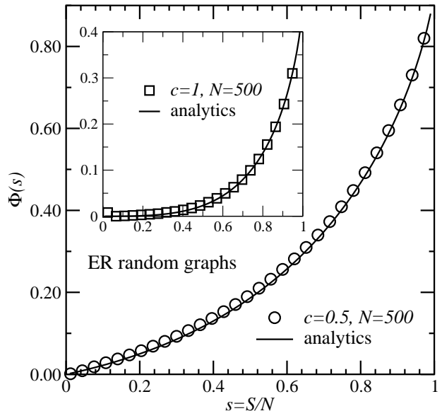
Fig. 2. Large-deviation rate function \Phi(s) of ER random graphs with average connectivity c = 0.5 < c_c , N = 500 (symbols). The line displays the analytical result from Eq. (2). The inset shows the same for the case c = 1.0 = c_c .
