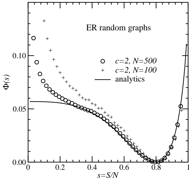
Fig. 3. Large-deviation rate function \Phi(s) of ER random graphs with average connectivity c = 2 > c_c , N = 100 and N = 500 (symbols). The line displays the analytical result from Eq. (2).
