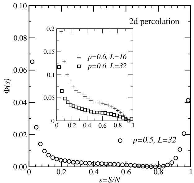
Fig. 8. Large-deviation rate function \Phi(s) of two-dimensional (2d) bond percolation with occupation probability p = 0.5 = p_c , L = 32 and (inset) p = 0.6 , L = 16/L = 32 .
