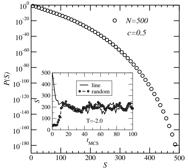
Fig. 1. Distribution of the size S of the largest component for Erdős-Rényi random graphs of size N = 500 at connectivity c = 0.5 . In this and all other plots, error bars are of symbol size or smaller if not explicitly shown. The inset shows the size of the largest component as function of the number t_{\text{MCS}} of Monte Carlo sweeps for the same type of graphs at temperature T = -2 . Two different starting conditions are displayed: either a random graph (leading to a typical components size around 30) or a graph consisting of a line ( S = 500 ) were used.
