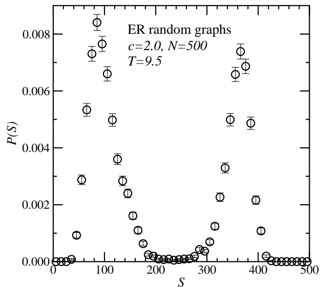
Fig. 6. Distribution (normalised such that the integral is one) of the size of the largest component for ER random graphs ( c = 2 , N = 500 ) at artificial temperature T = 9.5 .
