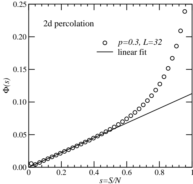
Fig. 7. Large-deviation rate function \Phi(s) of two-dimensional (2d) bond percolation with occupation probability p = 0.3 < p_c , L = 32 (symbols). For small relative cluster sizes s , the rate function behaves linearly (the line displays a linear function with slope 0.1125, obtained from fitting a linear function to the data in the range s \in [0, 0.5] ).
