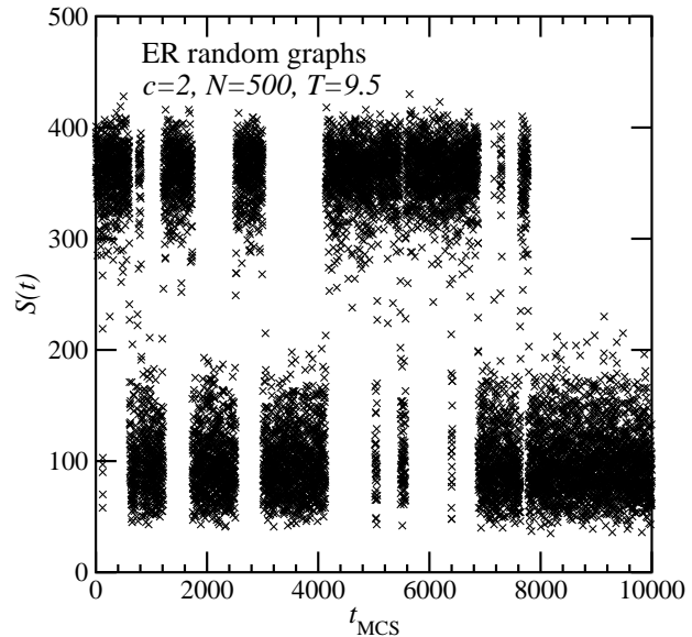
Fig. 5. Time-series for the size S of largest cluster as function of the number t_{\text{MCS}} of MC sweeps for ER random graphs ( c = 2 , N = 500 ) at artificial temperature T = 9.5 .
