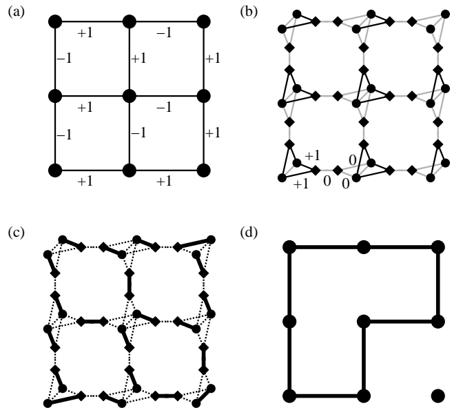
FIG. 2: Illustration of the algorithmic procedure: (a) original lattice G with edge weights, (b) auxiliary graph G_A with proper weight assignment. Black edges carry the same weight as the respective edge in the original graph and grey edges carry zero weight, (c) minimum-weight perfect matching (MWPM) M : bold edges are matched and dashed edges are unmatched, and (d) loop configuration (bold edges) that corresponds to the MWPM depicted in (c).
