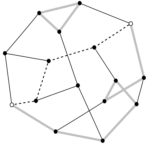
FIG. 1: Example of a r -regular random graph with N = 16 nodes and fixed degree r = 3 . The depicted graph has a diameter R_{N,r} = 4 , where the diameter is the longest among all shortest paths (measured in node-to-node hops). For a given realization of the quenched disorder, the negative-weight percolation algorithm might yield the path+loop configuration illustrated by means of the bold gray edges. Therein, a path is forced to join two distinguished nodes (open circles) that are maximally separated, i.e. have distance R_{N,r} . The dashed path corresponds to a shortest path joining the two distinguished nodes.
