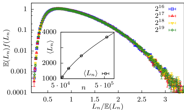
FIG. 7. Data collapse of the distributions with the optimal pair (a,b) = (0.36, 0.36) that minimizes S_{a,b} . The inset shows the empirical averages \langle L_n \rangle and their prediction according to Eq. (20) with the optimal constants (a,b) = (0.36, 0.36) .
