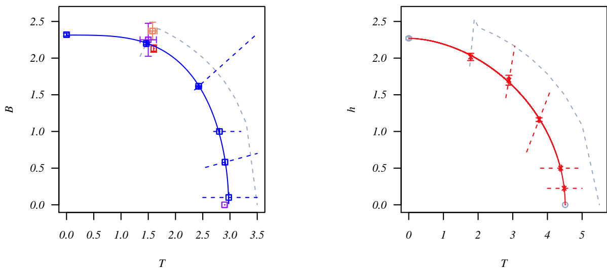
FIG. 5: (Color online) Left: Empirical phase boundary of the DAFF ( p = 0.7 ). The red point is from Ref. 38, the coral point from Ref. 39, and the purple points from Ref. 40. Our data agree within error bars with these previous studies. The blue (solid) curve is given by Eq. (13). The dashed lines represent the parts of the simulation paths that cross the phase boundary. The light shaded line is an example of the second RC that runs parallel to the approximated phase boundary to a temperature T > T_c and B = 0 to speed up equilibration. Right: Empirical phase boundary of the RFIM. The zero-field critical temperature is T_c^0 = 4.5115^{41} and h_c^0 = 2.270^{42} (grey open circles). The red (solid) curve is given by Eq. (14). The dashed lines represent the parts of the simulation paths that cross the phase boundary. Again, the light shaded line shows an example of the second RC that runs parallel to the approximated phase boundary to a temperature T > T_c and h = 0 to speed up equilibration.
