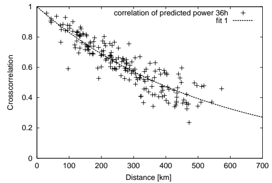
Figure 4: Crosscorrelation of 36 hour prediction of power for each pair of sites.
