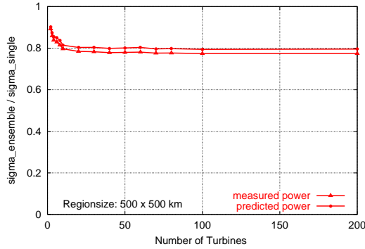
Figure 5: Ratio between standard deviation of regional power and single power versus number of sites for a region of 500 \times 500 \text{ km}^2
