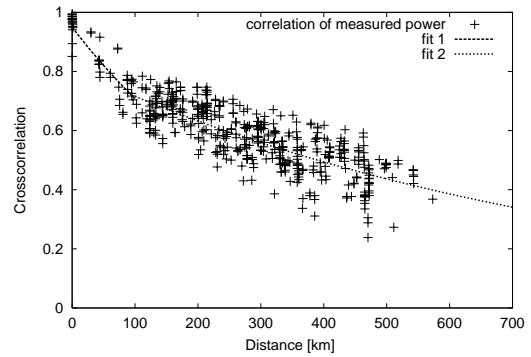
Figure 3: Crosscorrelation of measured power for each pair of sites.
