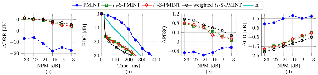
Fig. 4. Performance of the PMINT technique and sparsity-promoting PMINT technique using different penalty functions for acoustic system S_1 in terms of (a) \Delta DRR, (b) EDC for an exemplary NPM of -33 dB, (c) \Delta PESQ, and (d) \Delta CD (intrusively selected weighting and penalty parameters \eta and \rho ).
