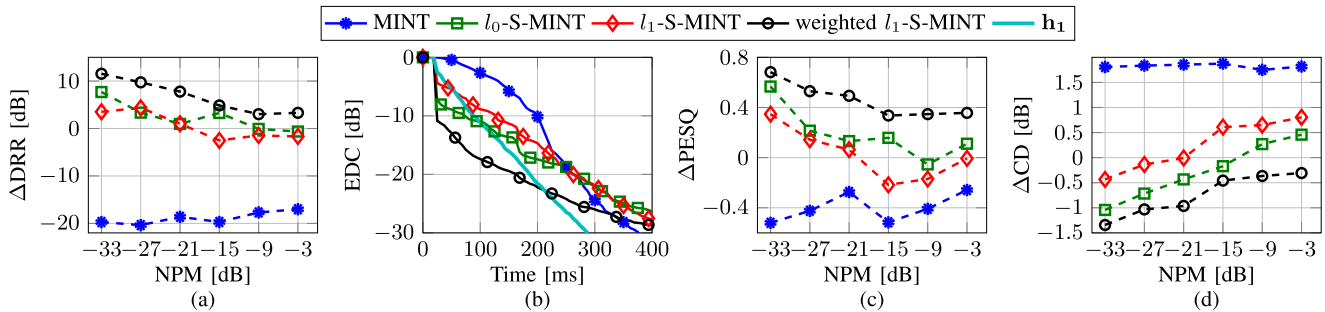
Fig. 2. Performance of the MINT technique and sparsity-promoting MINT technique using different penalty functions for acoustic system S_1 in terms of (a) \Delta DRR, (b) EDC for an exemplary NPM of -33 dB, (c) \Delta PESQ, and (d) \Delta CD (intrusively selected weighting and penalty parameters \eta and \rho ).
