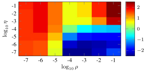
Fig. 6. Performance of the weighted l_1 -norm sparsity-promoting PMINT technique in terms of \Delta CD for several weighting and penalty parameters \eta and \rho (acoustic system S_1 , NPM = -33 dB).
