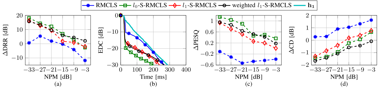
Fig. 3. Performance of the RMCLS technique and sparsity-promoting RMCLS technique using different penalty functions for acoustic system S_1 in terms of (a) \Delta DRR, (b) EDC for an exemplary NPM of -33 dB, (c) \Delta PESQ, and (d) \Delta CD (intrusively selected weighting and penalty parameters \eta and \rho ).
