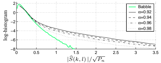
Fig. 2. Log-histogram of the filtered spectrum |\hat{S}(k, l)| for babble noise. For comparison, the histogram of scaled unfiltered babble noise ( \hat{S}(k, l) = G_{\min} N(k, l) ) is also given. Due to high fluctuations in the noise, the number of outliers can hardly be controlled by the choice of \alpha .
