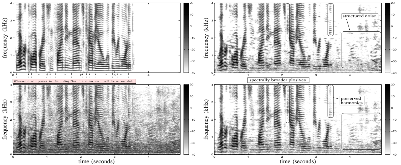
Fig. 5. Comparison of spectrograms. The sentence is “Whoever cooperates in finding Nan’s cameo will be rewarded”. On the left, the clean (top) and the unfiltered signal (bottom) are shown. The noise is babble noise at an SNR of 0dB. On the right, the filtered signals are given. The conventional filter (top) causes more noise fluctuations than the filter with cepstral smoothing (bottom). At the same time, cepstral smoothing preserves the structure of speech better.
