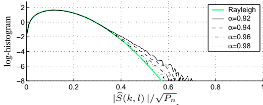
Fig. 3. Log-histogram of the filtered spectrum |\hat{S}(k, l)| for Gaussian noise as in Figure 1 but with cepstral smoothing applied. Cepstral smoothing reduces the number of outliers considerably. The residual noise sounds like Gaussian noise.
