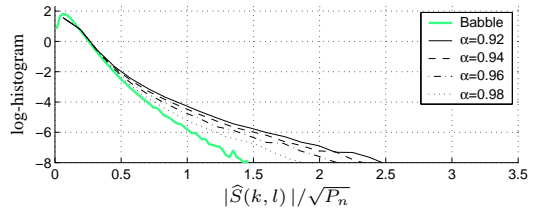
Fig. 4. Log-histogram of the filtered spectrum |\hat{S}(k, l)| for babble noise as in Figure 2 but with cepstral smoothing applied. The residual noise sounds more natural, as spectral outliers are less pronounced.
