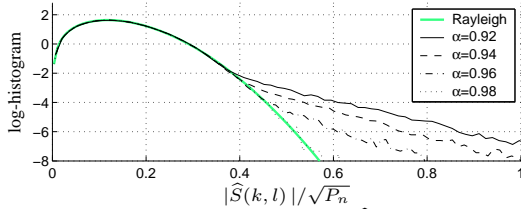
Fig. 1. Log-histogram of the filtered spectrum |\hat{S}(k, l)| for Gaussian noise. For comparison, the Rayleigh pdf of the magnitude of Gaussian noise is also given. The lower the smoothing constant \alpha , the more spectral outliers can be observed. The outliers of relatively large amplitude are perceived as musical noise .
