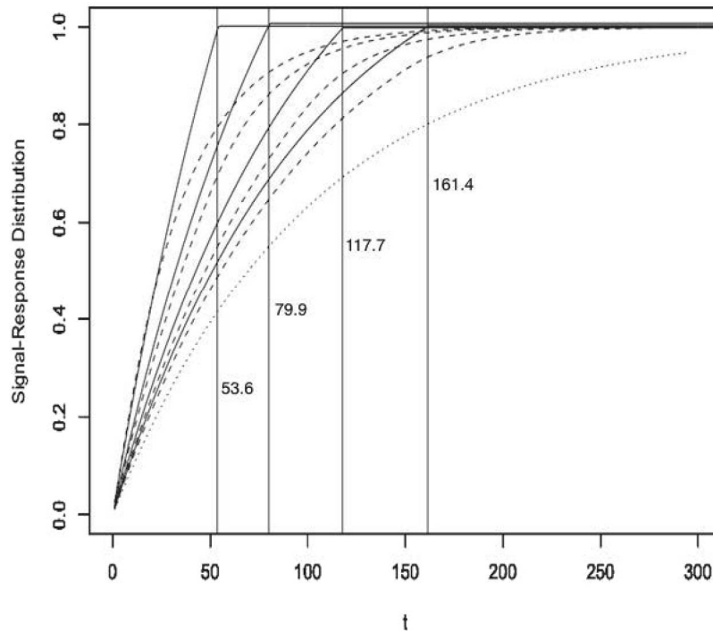
Figure 1. The “fan” effect: All signal-response reaction time distributions F_{sr}(t|t_d) are strictly ordered by delay ( t_d ) from left to right, for t_d = 10, 50, 100, and 150 ms, converging toward no-stop signal distribution F_{go}(t) (rightmost curve) for t_d \rightarrow \infty , for exponential distributions with rate parameters \lambda_{go} = .01 and \lambda_{stop} = .02 . The vertical lines and their corresponding g^{-1}(t_d) values indicate the crossing points where F_{sr}(t|t_d) = 1 for the PND model. The PND model curves were obtained by simulation (see Appendix); dashed: IND model; solid: PND model. PND = perfect negative stochastic dependence; IND = independent race model.
