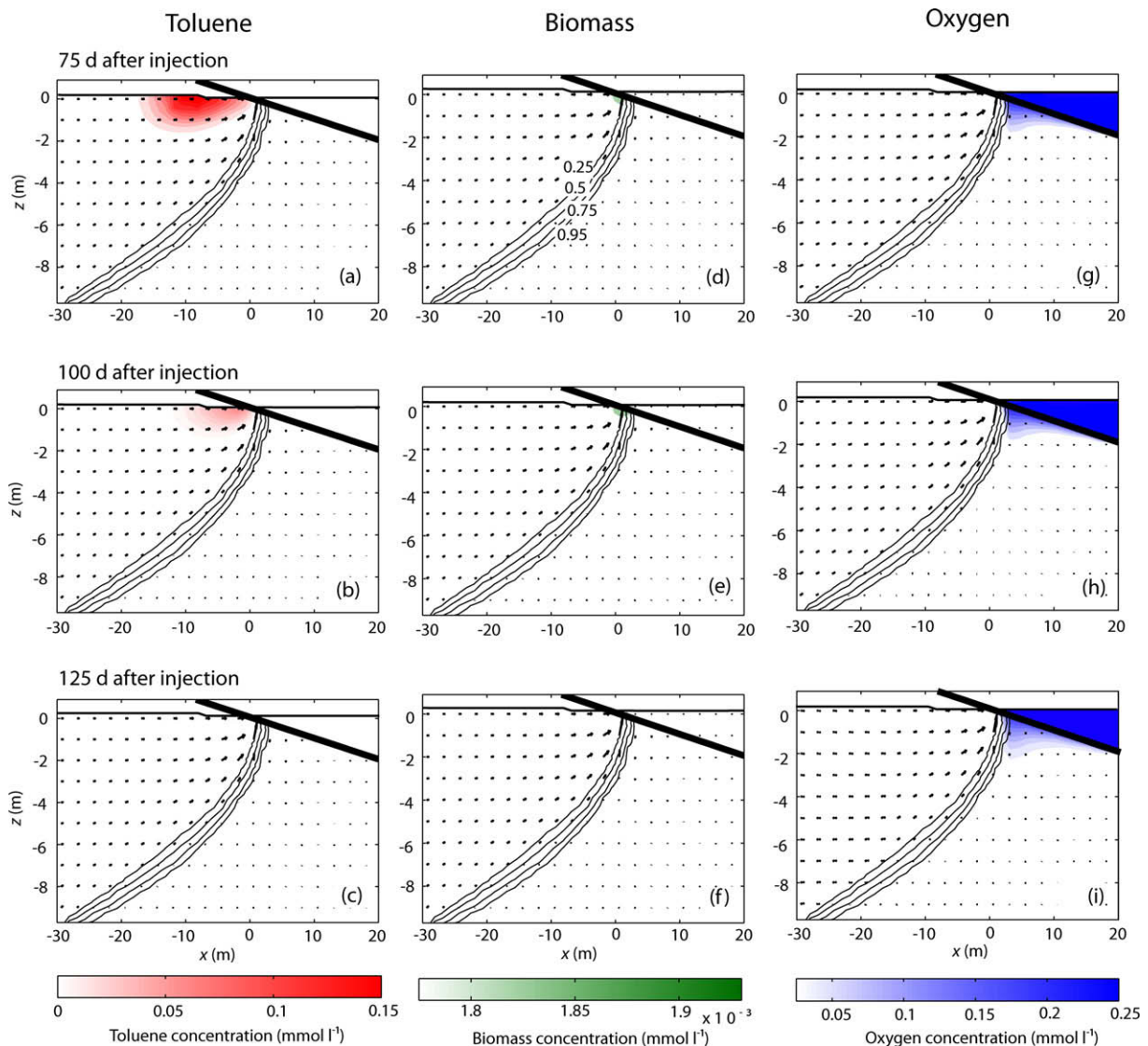
Fig. 3. Concentrations of toluene (a–c), biomass (d–f) and oxygen (g–i) 75, 100 and 125 d after injection of toluene for simulation with aerobic biodegradation and b_o = 0.09 \text{ d}^{-1} but no tidal forcing. The arrows represent the steady state flow. The contour lines depict the salt distribution in the near-shore aquifer where the contour levels (fraction seawater) are the same for all subplots and are notated in (d). Note that there is only minor biomass growth close to the shoreline (evident 75 and 100 d after injection) for these conditions.
