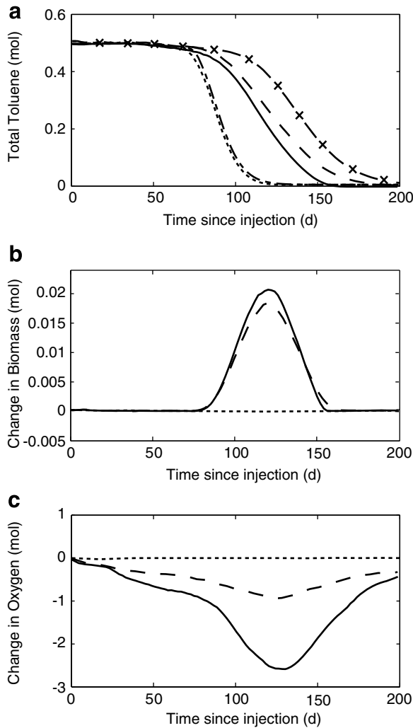
Fig. 5. (a) Total moles of toluene, (b) change in total moles of biomass and (c) change in total moles of oxygen in the aquifer following toluene injection for simulations without tides and without biodegradation (---), without tides but with biodegradation and b_o = 0.09 \text{ d}^{-1} (···), with tides but without biodegradation ( - \times - ), with tides, biodegradation and b_o = 0 \text{ d}^{-1} (—) and with tides, biodegradation and b_o = 0.09 \text{ d}^{-1} (—).
