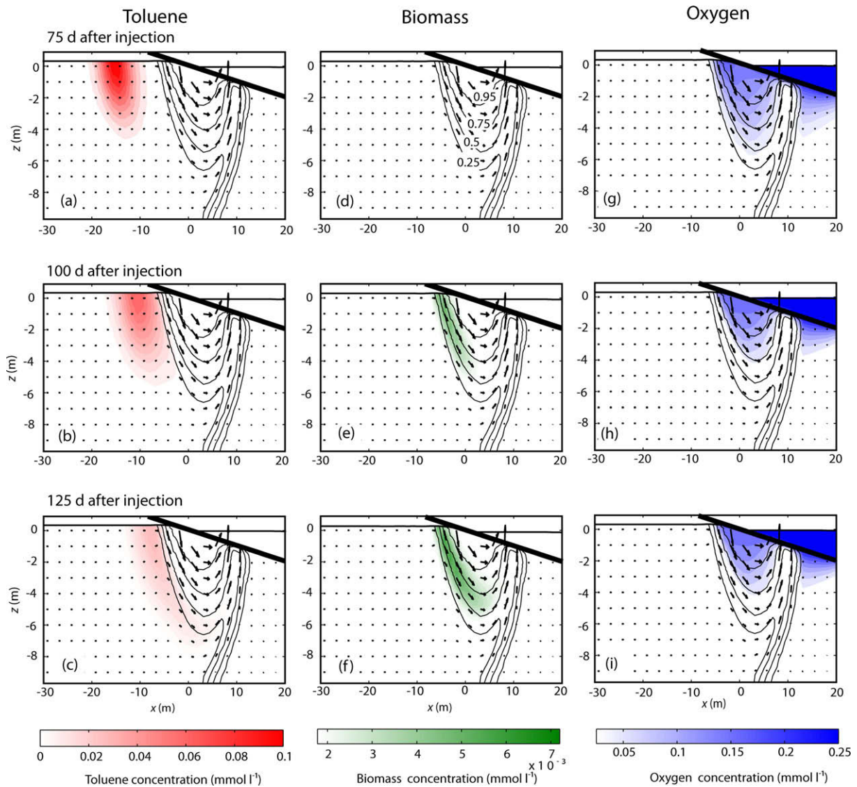
Fig. 4. Concentrations of toluene (a–c), biomass (d–f) and oxygen (g–i) 75, 100 and 125 d after injection of toluene for simulation with tidal forcing, aerobic biodegradation and b_0 = 0.09 \text{ d}^{-1} . The arrows represent the tide-averaged groundwater flow. The contour lines depict the salt distribution in the near-shore aquifer where the contour levels (fraction seawater) are the same for all subplots and are noted in (d).
