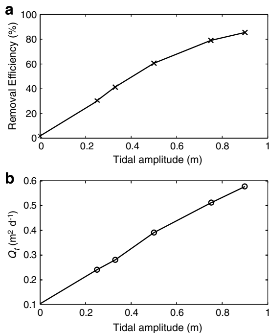
Fig. 9. Influence of tidal amplitude on (a) the removal efficiency of toluene in the subsurface prior to discharge and (b) Q_t (tidally driven seawater recirculation).
