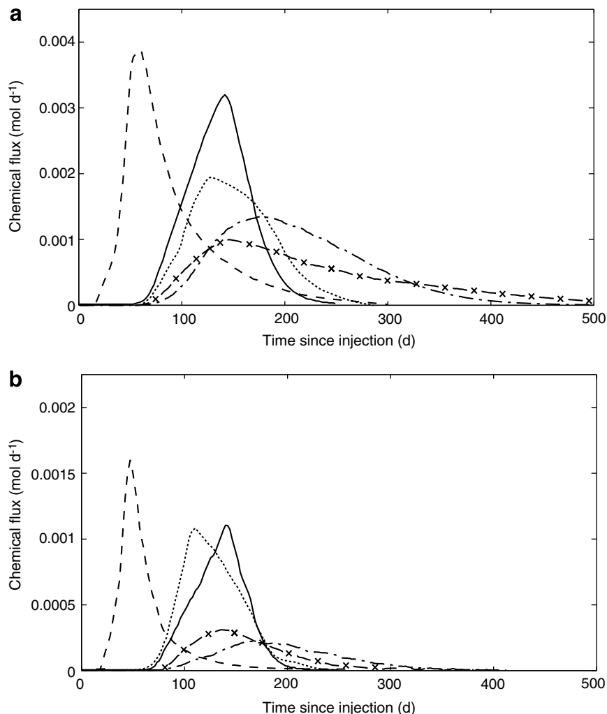
Fig. 12. Total toluene flux across the aquifer–ocean interface versus time since toluene injection (a) without biodegradation and (b) with biodegradation for homogeneous aquifer conditions (—) and heterogeneous conductivity fields 1 (---), 2 (-·-·), 3 (···) and 4 (- - -). Note the change in vertical scale between (a) and (b).
