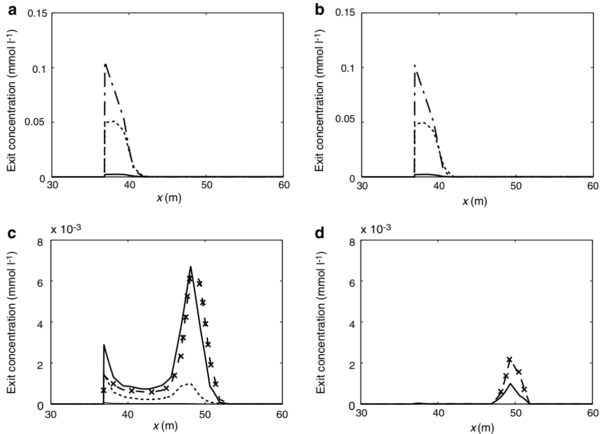
Fig. 7. Toluene exit concentrations along the aquifer–ocean interface for simulations (a) without tides and without biodegradation, (b) without tides but with biodegradation, (c) with tides but without biodegradation and (d) with tides and with biodegradation. Results are shown for 75 d (---), 100 d (···), 125 d (—) and 150 d (– · –) after toluene injection. Note the changes in vertical scale.
