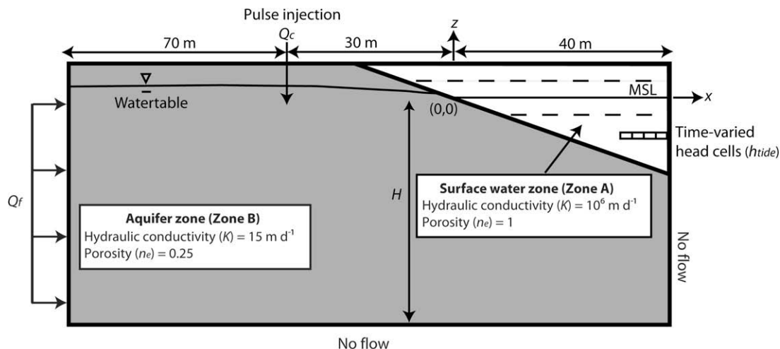
Fig. 2. Model geometry and boundary conditions. The model domain is divided into two zones: a surface water zone (zone A, not shaded) and an aquifer zone (zone B, shaded).
