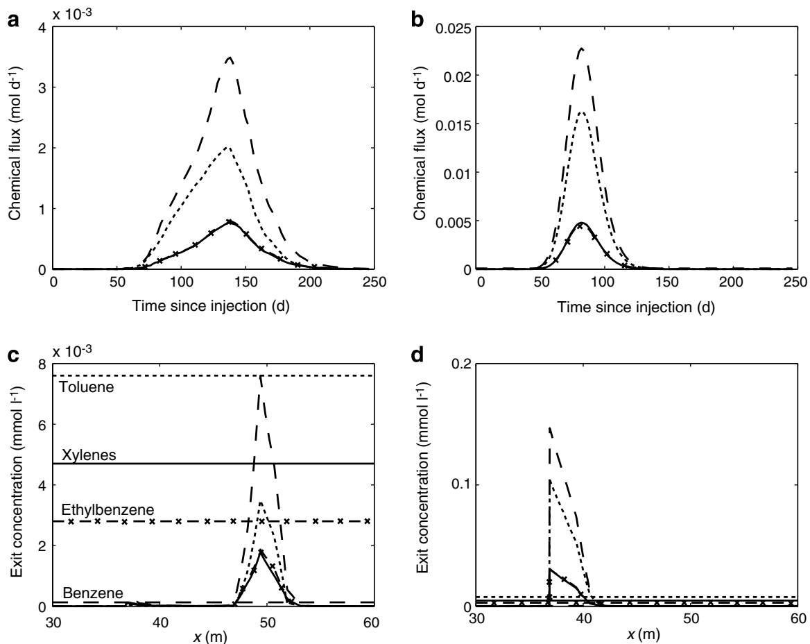
Fig. 8. Total flux of benzene (---), toluene (···), ethylbenzene (- × -) and xylenes (-) across the aquifer–ocean interface versus time since BTEX injection for simulations (a) with and (b) without tides. The exit concentrations along the aquifer–ocean interface for each component (c) 140 d after BTEX injection with tides present and (d) 80 d after BTEX injection in the absence of tides are also shown. The WHO guideline concentrations [42] for benzene ( 0.13 \mu\text{mol l}^{-1} ), toluene ( 7.6 \mu\text{mol l}^{-1} ), ethylbenzene ( 2.8 \mu\text{mol l}^{-1} ) and xylenes ( 4.7 \mu\text{mol l}^{-1} ) are indicated in (c) and (d). Note the change in vertical scale between (c) and (d).
