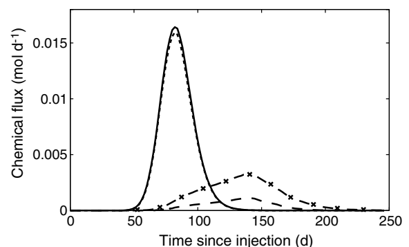
Fig. 6. Total toluene flux across the aquifer–ocean interface versus time since toluene injection for simulation without tides and without biodegradation (—), without tides but with biodegradation (···), with tides but without biodegradation ( - \times - ) and with tides and biodegradation (—). For all simulations b_o = 0.09 \text{ d}^{-1} .
