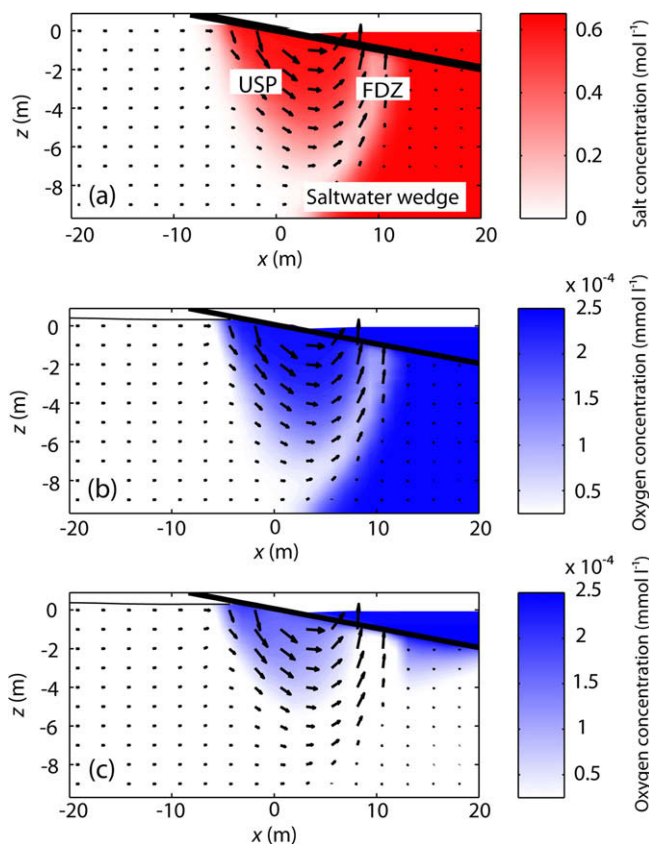
Fig. 1. Simulated (a) salt distribution, (b) oxygen distribution with no natural oxygen-consuming processes ( b_o = 0 ) and (c) oxygen distribution with natural oxygen consumption ( b_o = 0.09 \text{ d}^{-1} ) in a tidally influenced near-shore aquifer (base conditions). The upper saline plume (USP), saltwater wedge and freshwater discharge zone (FDZ) are denoted in (a). The arrows represent the groundwater flows averaged over a tidal cycle.
