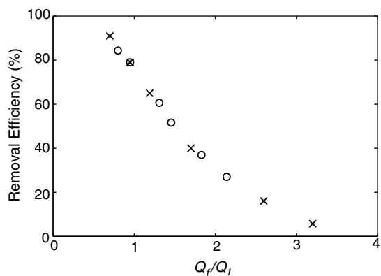
Fig. 10. Relationship between Q_f/Q_t (ratio of fresh groundwater discharge to tidally driven seawater recirculation) and the removal efficiency of toluene in the subsurface prior to discharge. Circles indicate results from simulations with tidal amplitude varied from the base conditions and crosses indicate results from simulations with Q_f varied from the base conditions.
