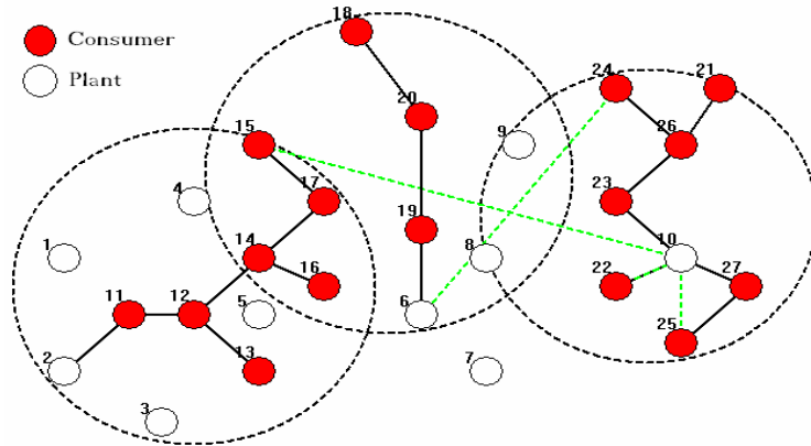
Figure 1: Final solution of the Test Scenario after 100 iterations using 20 ants
