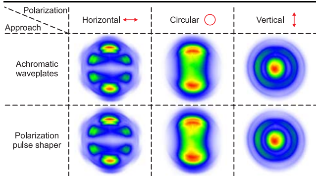
Fig. 7 Measured PADs from excitation of potassium with femtosecond laser pulses being in different states of polarization. The pulses were generated using two different methods: achromatic waveplates ( upper row ) and the polarization pulse shaper ( lower row ). The agreement between both approaches is excellent
