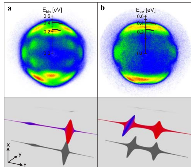
Fig. 11 Upper panels : measured PADs from excitation with linearly polarized phase-shaped laser pulses of 280 nJ pulse energy. Lower panels : three-dimensional visualization of the shaped pulses in the laboratory frame. Note that the time axis corresponds to the negative z -axis. (a) the spectral phase function \varphi_V(\omega) = -200 \text{ fs} \cdot |\omega - 2.44 \text{ fs}^{-1}| generates a weak blue-detuned pre-pulse followed by an intense red-detuned post-pulse separated by 400 fs, whereas (b) the spectral phase function \varphi_V(\omega) = -200 \text{ fs} \cdot |\omega - 2.36 \text{ fs}^{-1}| generates a blue-detuned pre-pulse followed by a red-detuned post-pulse of almost equal intensity
