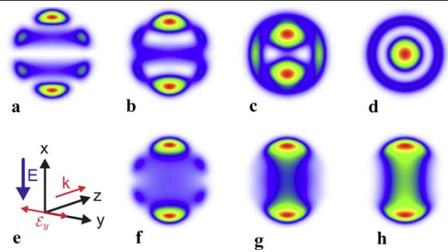
Fig. 3 Simulated PADs for \Theta = 2\pi pulses. Upper panels: \mathcal{E}_L = -\mathcal{E}_R , with relative phases of (a) 0, (b) \pi/3 , (c) 2\pi/3 , and (d) \pi ( \mathcal{E}_L = \mathcal{E}_R ) corresponding to light pulses linearly polarized with an angle of 0^\circ , 30^\circ , 60^\circ , and 90^\circ with respect to the y -axis (compare to the experimental PADs in Fig. 10(a)–(d)). Lower panels left: (e) sketch of the coordinate system for the simulation. The extraction field E along the x -axis determines the direction of the Abel-transform and the k -vector along the z -axis describes the light propagation direction. \mathcal{E}_y describes light polarized along the y -axis. Lower panels right: variation of the relative amplitude and phase of the left and right circularly polarized light fields mimicking the effect of elliptically polarized light from a \lambda/4 plate with retardation axis oriented at (f) 15^\circ , (g) 30^\circ , and (h) 45^\circ with respect to the y -axis (compare with the experimental PADs in Fig. 10 (e)–(h))
